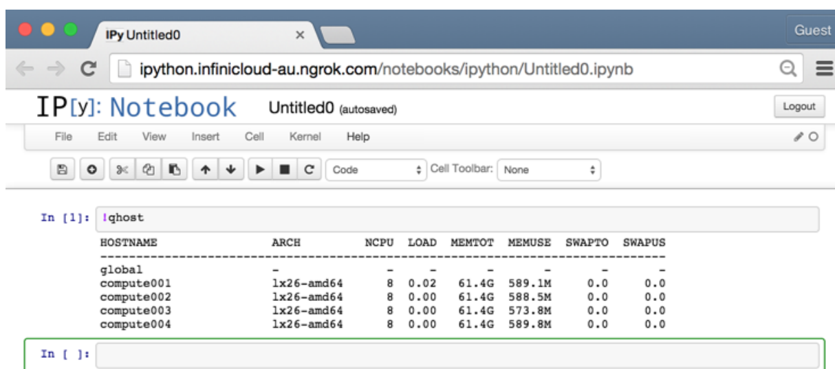
Figure 7. IPython notebook
